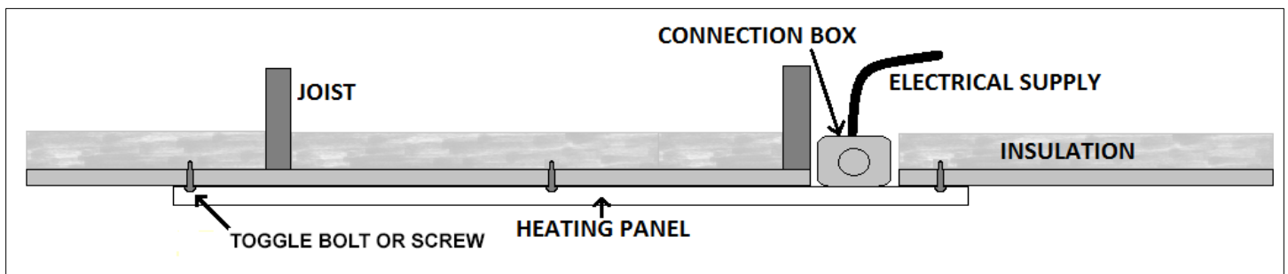
Figure 1 – Surface Mounting
