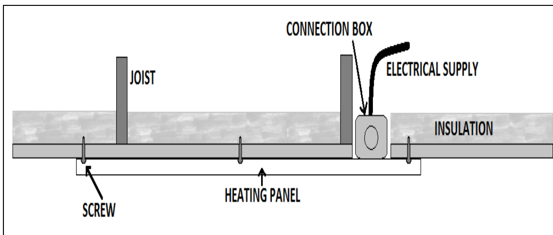
Figure 1 – Surface Mounting
